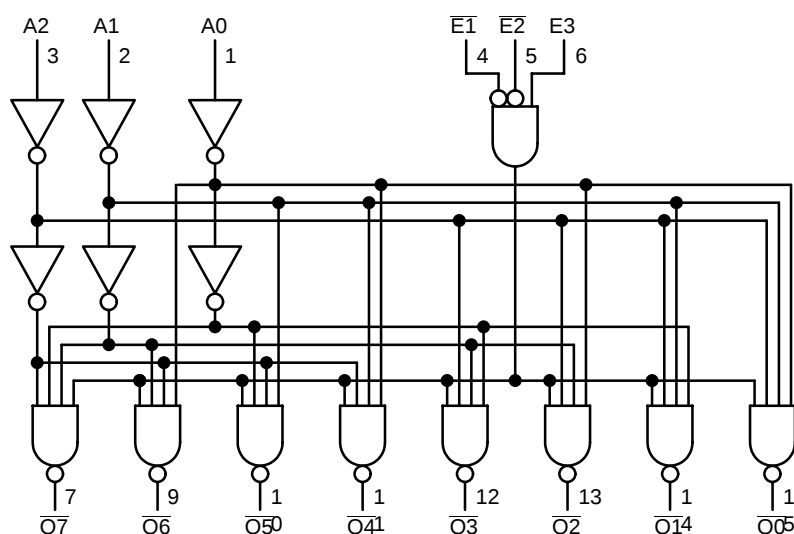
Figure 2. Logic Diagram
