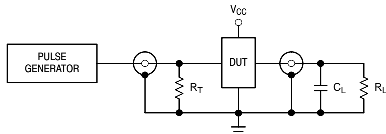
Figure 3. AC Waveforms
