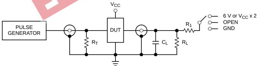
Figure 4. Test Circuit
