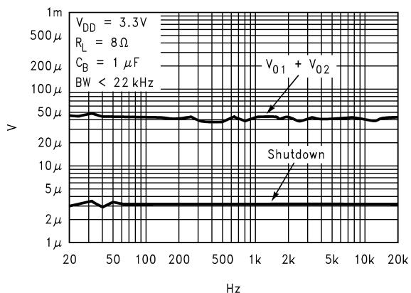
Noise Floor
