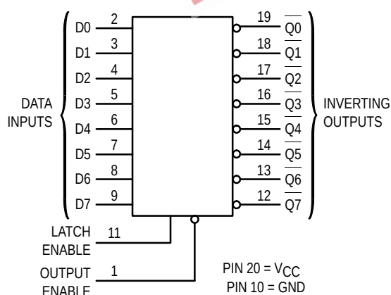
LOGIC DIAGRAM
