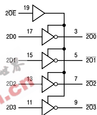
Figure 2. LOGIC DIAGRAM
