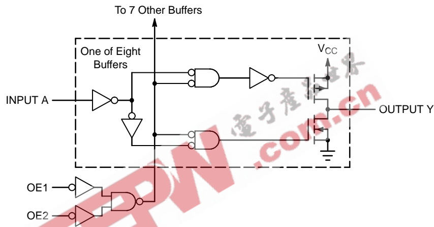
Figure 7. Logic Detail
