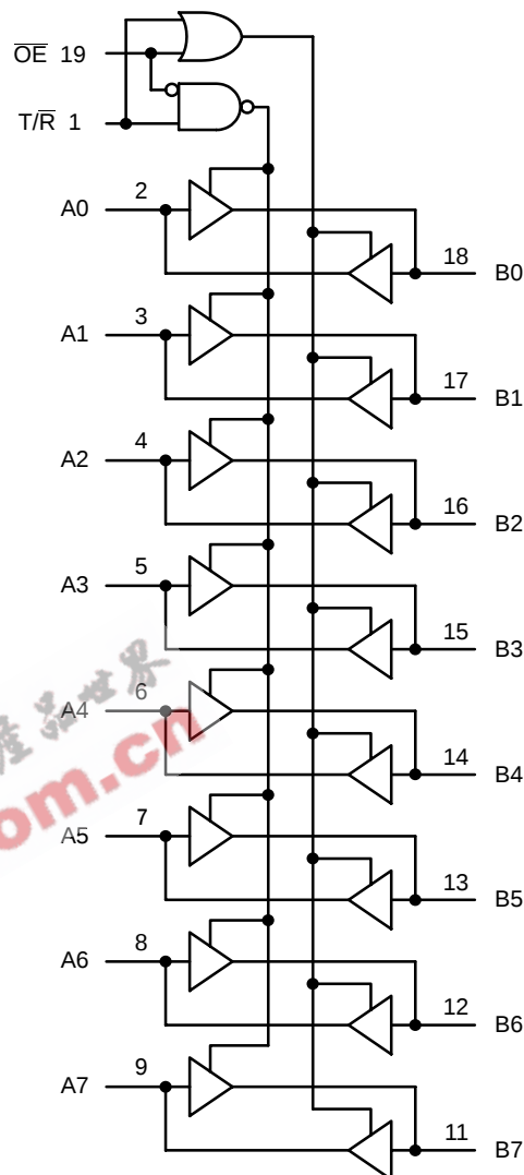
Figure 2. Logic Diagram
