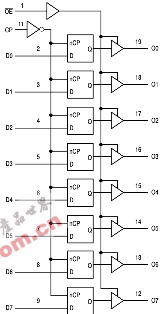
Figure 2. LOGIC DIAGRAM
