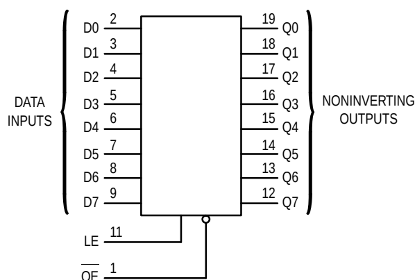
LOGIC DIAGRAM
