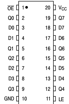
Figure 2. Pin Assignment
