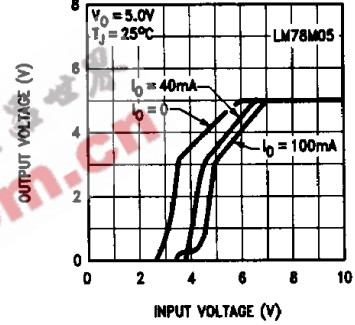
Dropout Characteristics
