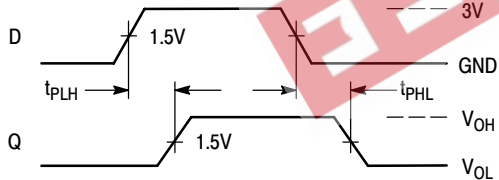
Figure 3. Switching Waveform
