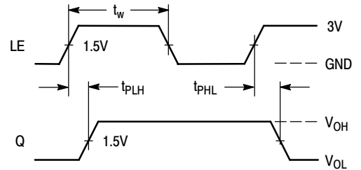
Figure 4. Switching Waveform
