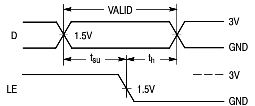
Figure 6. Switching Waveform
