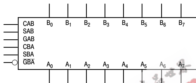
Figure 6. Logic Symbol
