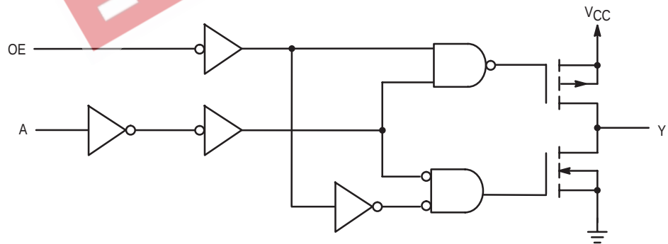
HC125A (1/4 OF THE DEVICE)
