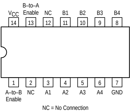
Pinout: 14-Lead Plastic Package (Top View)
