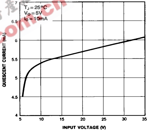
Figure 4. Quiescent Current
