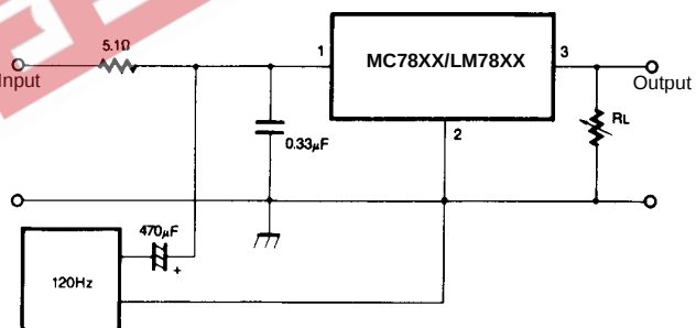
Figure 7. Ripple Rejection
