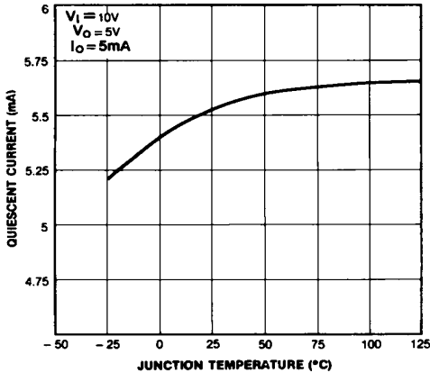
Figure 1. Quiescent Current
