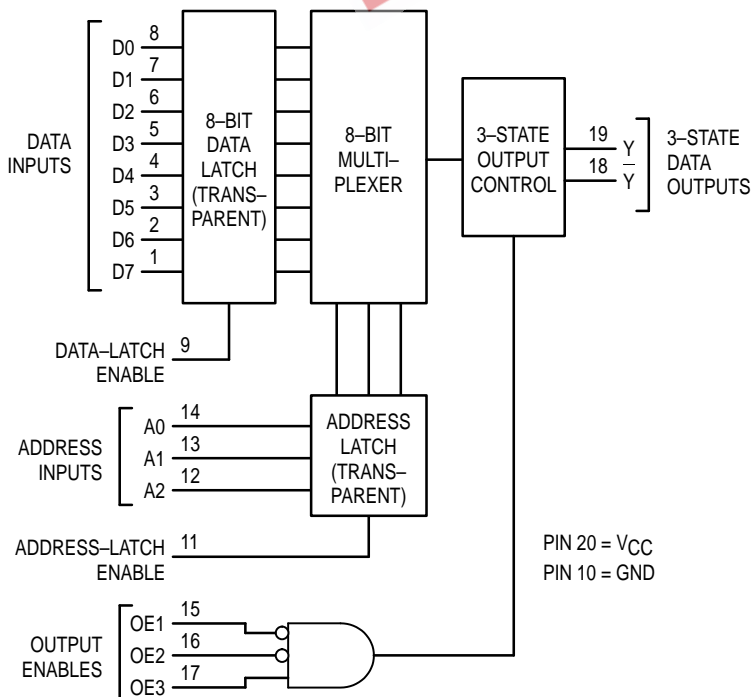
LOGIC DIAGRAM
