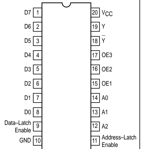
Pinout: 20-Lead Package (Top View)
