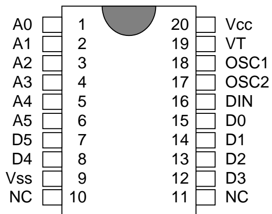
SM5272BS-M6/L6
