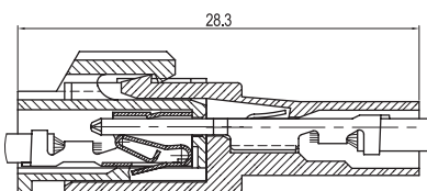
TERMINAL ASSEMBLY DRAWING
