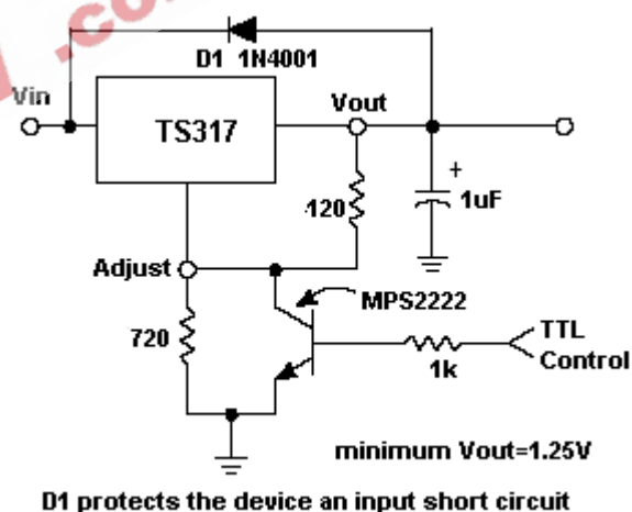
Figure 9. 5V electronic shutdown regulator
