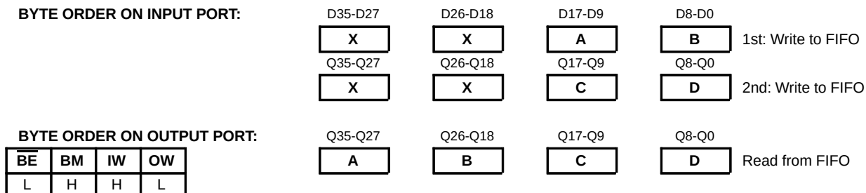
(a) ×18 INPUT TO ×36 OUTPUT – BIG ENDIAN
