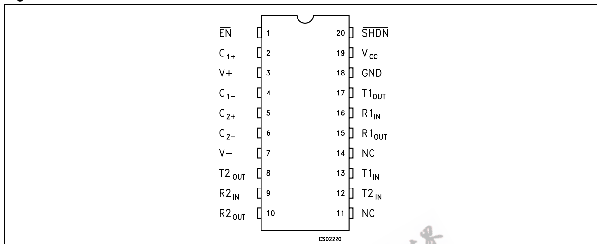
Figure 1. Pin connection
