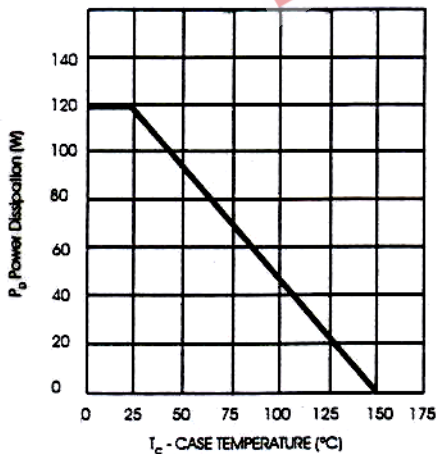
Figure 1, Power Derating
