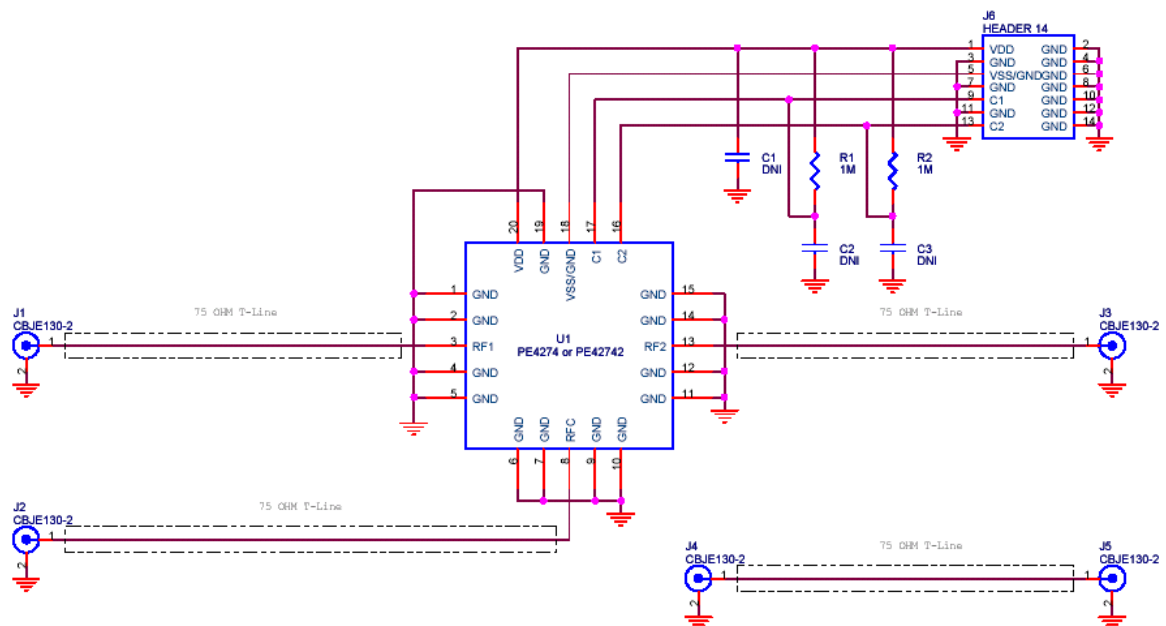
Figure 19. Evaluation Board
