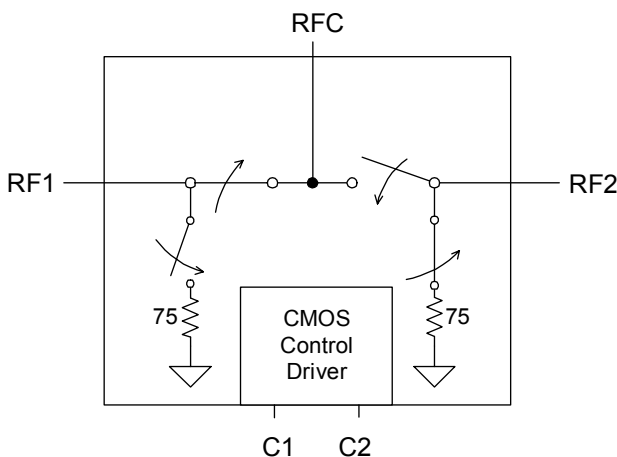
Figure 1. Functional Diagram
