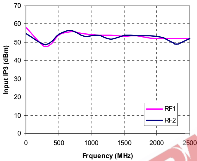
Figure 16. Input IP3: RFC-RF1/RF2
