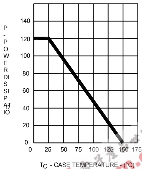
Figure 1. Power Derating
