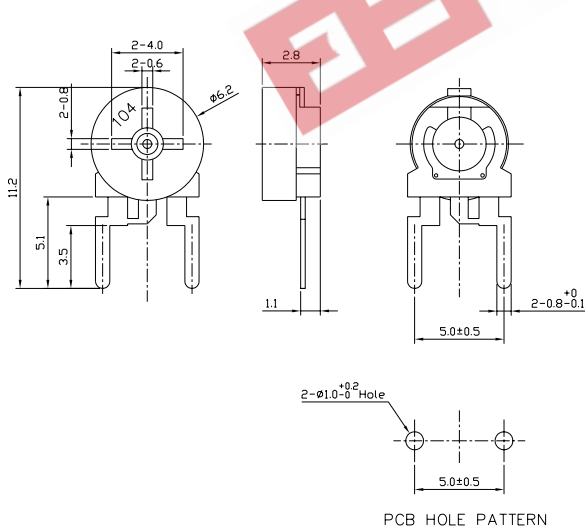
Model 40B (Side Adjust with 2 pins)
