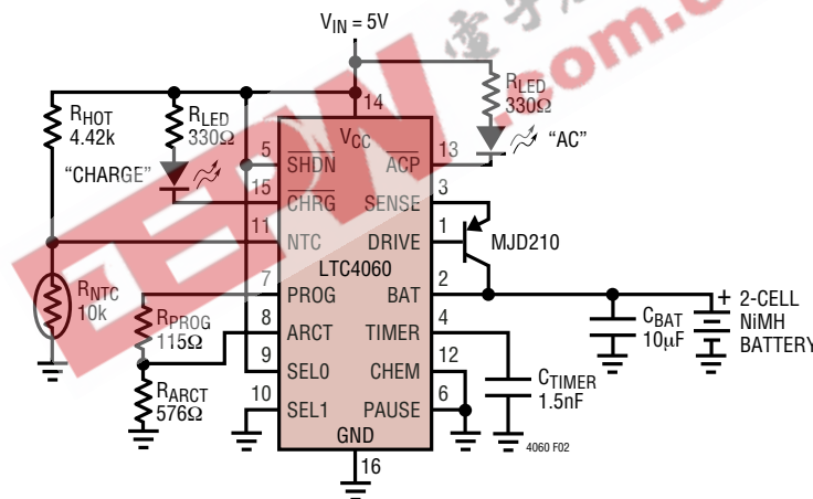
Figure 2. Full Featured 2A Charger Application
