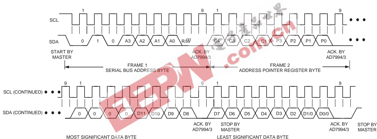
Figure 12. Two Byte Write Sequence
