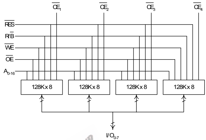
Logic Diagram
