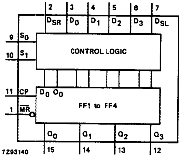
Fig.4 Functional diagram.
