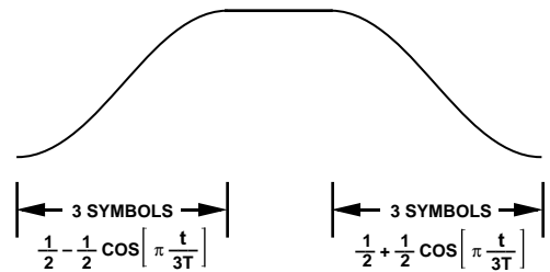
Figure 11. Ramp Envelope
