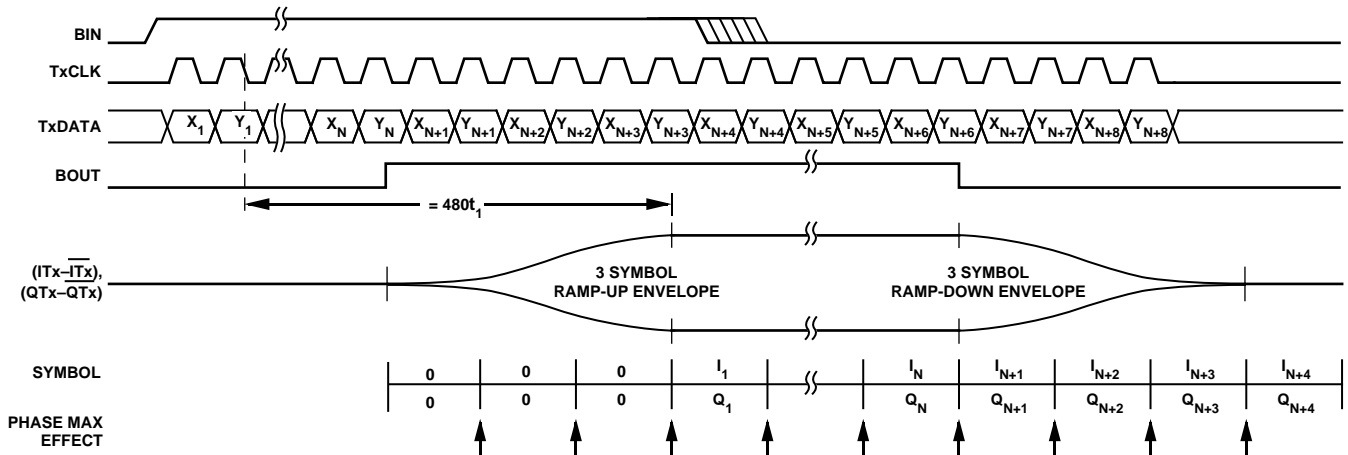
Figure 12. Transmit Burst
