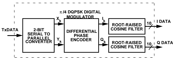
Figure 9. \pi/4 DQPSK Modulator Functional Block Diagram
