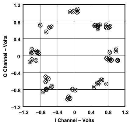
Figure 15. AD7011 Transmit Constellation Diagram
