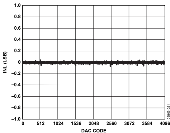
Figure 6. AD5024 INL
