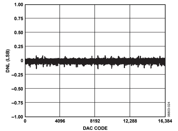
Figure 9. AD5024 DNL
