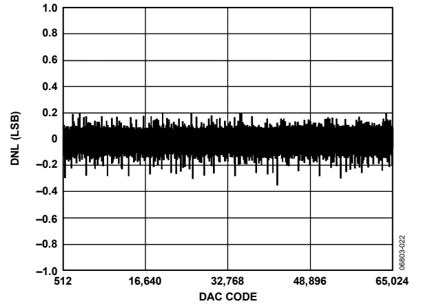
Figure 7. AD5064 DNL
