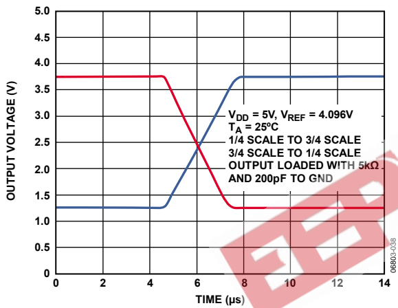
Figure 23. Settling Time
