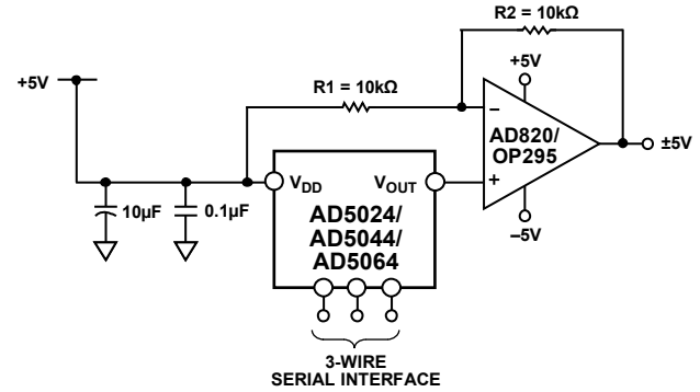
Figure 53. Bipolar Operation
