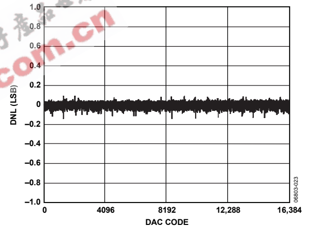
Figure 8. AD5044 DNL
