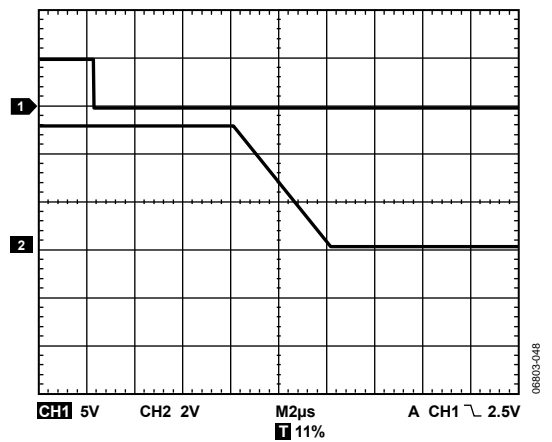
Figure 33. Hardware CLR
