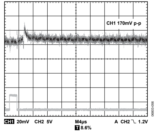
Figure 41. Glitch on Exiting Power-Down from Zero Scale, 5 kΩ/200 pF Load
