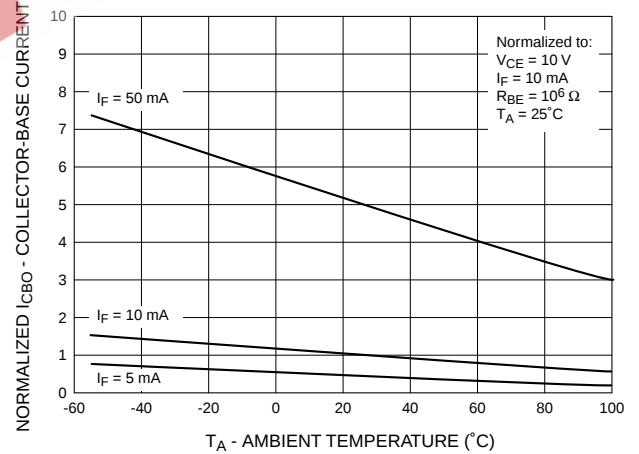
Normalized Collector-Base Current vs. Temperature
