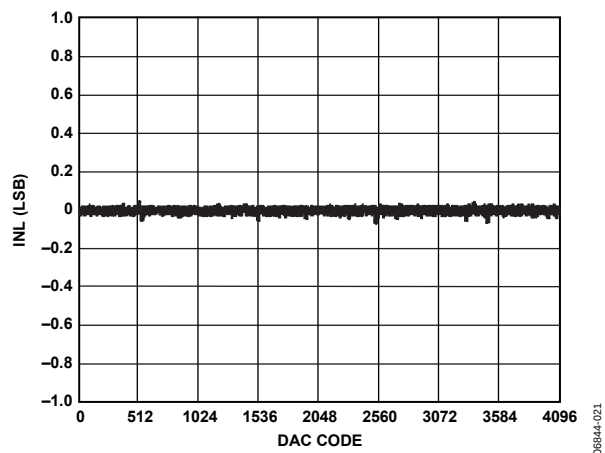
Figure 8. AD5025 INL
