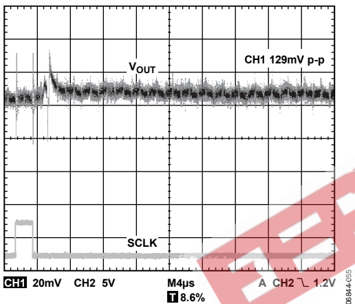
Figure 37. Glitch Upon Exiting Power-Down ( 1\text{ k}\Omega to GND) to Zero Scale, No Load
