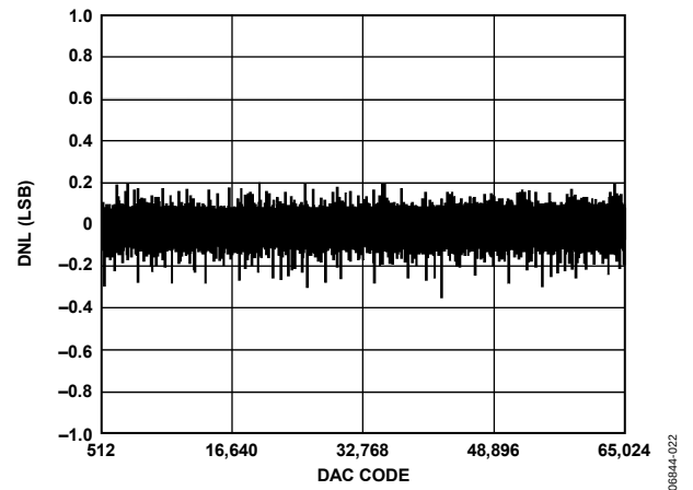
Figure 9. AD5065 DNL
