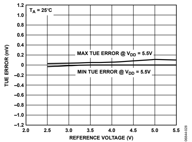
Figure 15. Total Unadjusted Error (TUE) vs. Reference Input Voltage
