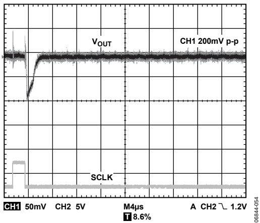
Figure 36. Glitch Upon Entering Power-Down ( 1\text{ k}\Omega to GND) from Zero Scale, 5\text{ k}\Omega/200\text{ pF} Load
