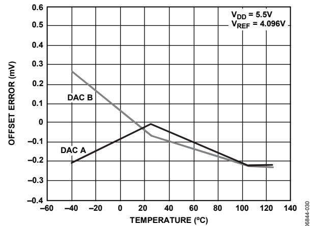
Figure 17. Offset Error vs. Temperature
