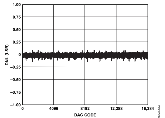
Figure 11. AD5025 DNL
