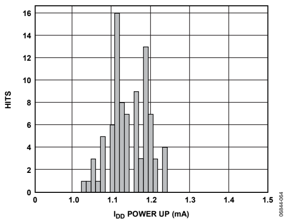
Figure 20. I_{DD} Histogram, V_{DD} = 5.0 V
