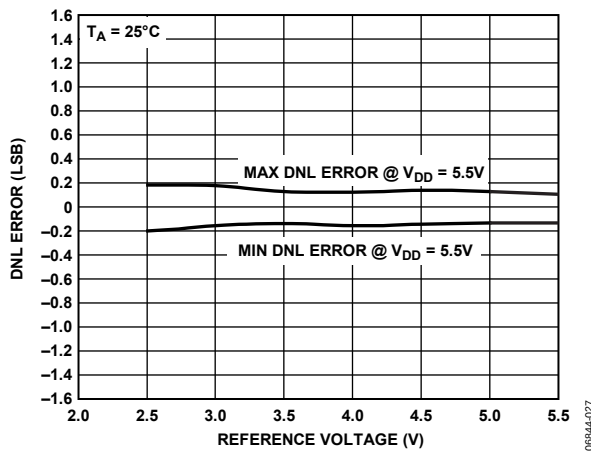
Figure 14. DNL vs. Reference Input Voltage
