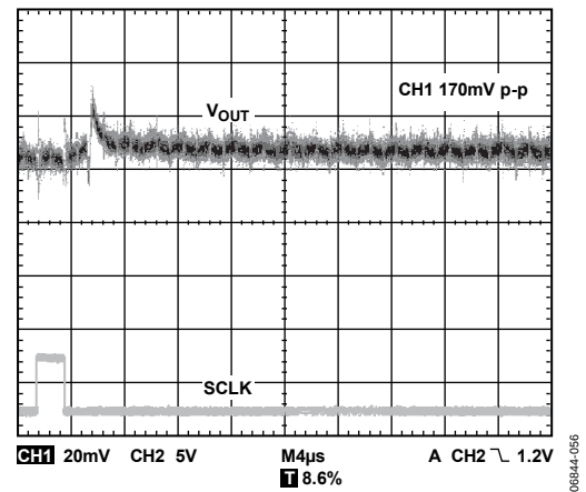
Figure 38. Glitch Upon Exiting Power-Down ( 1\text{ k}\Omega to GND) to Zero Scale, 5\text{ k}\Omega/200\text{ pF} Load
