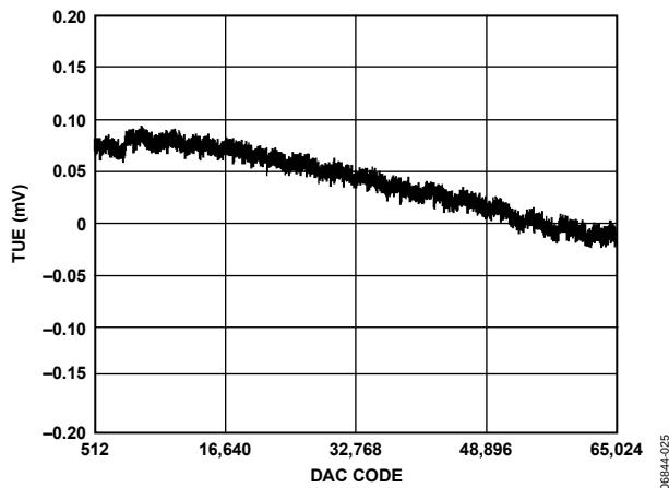
Figure 12. Total Unadjusted Error (TUE) vs. DAC Code
