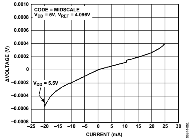
Figure 33. Typical Output Load Regulation
