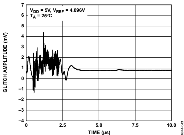
Figure 26. Analog Crosstalk
