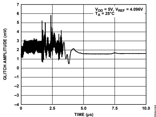
Figure 27. DAC-to-DAC Crosstalk
