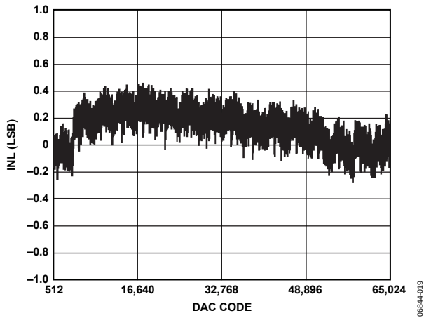
Figure 6. AD5065 INL
