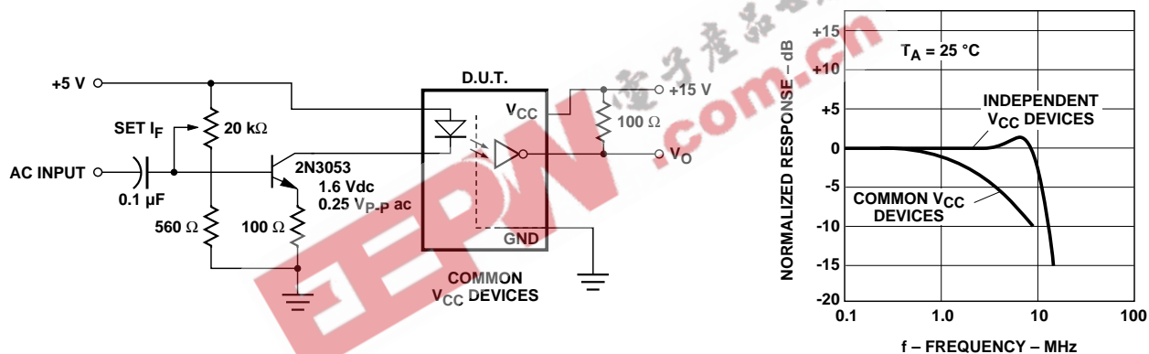
Figure 8. Frequency Response.
