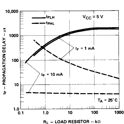
Figure 8. Propagation Delay vs. Load Resistor.
