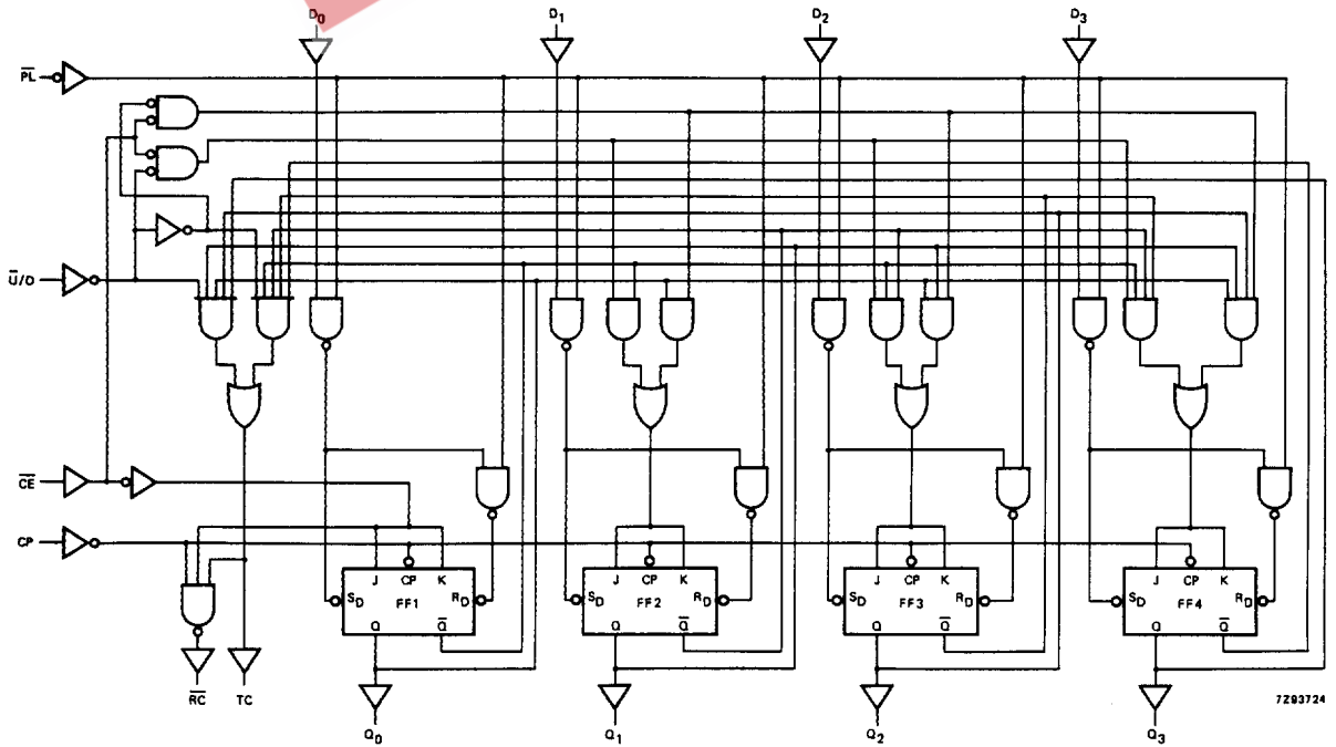
Fig.9 Logic diagram.
