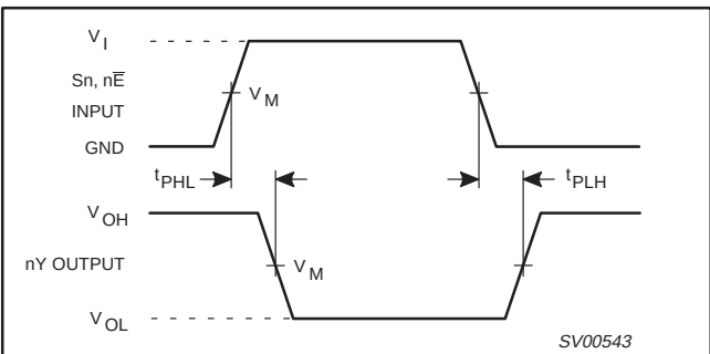
Figure 2. Select input ( S_0 , S_1 ) and the output enable input ( \bar{E} ) to output ( nY_n ) propagation delays.
