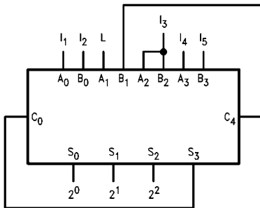
FIGURE 4. 5-Input Encoder
