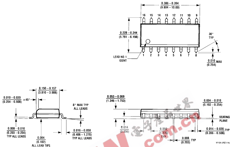
16-Lead Small Outline Molded Package (M) Order Number DM74LS169AM Package Number M16A
