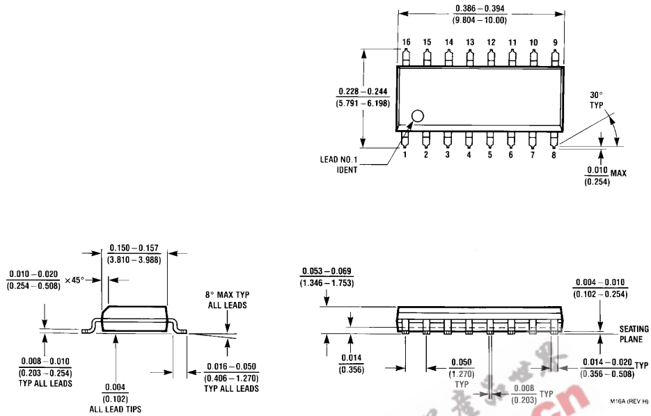
16-Lead Wide Small Outline Molded Package (M) Order Number DM74LS395WM NS Package Number M16B
