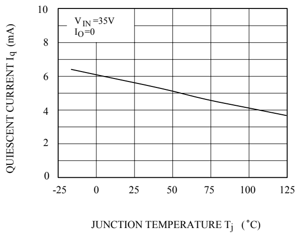
Fig.9 T_j - I_q
