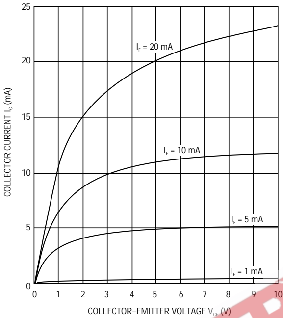
FIG. 5 - Collector Current vs. Collector-Emitter Voltage
