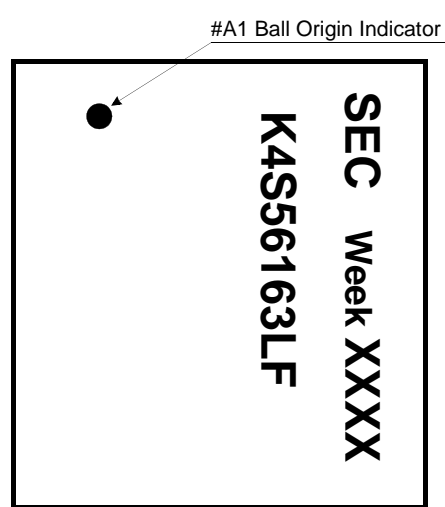
< Top View *2 >
