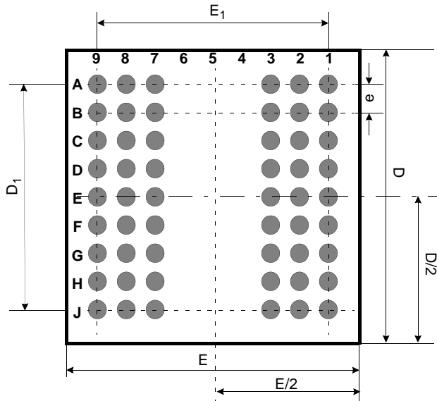
*2: Top View
