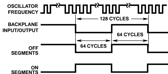
FIGURE 8. DISPLAY WAVEFORMS
