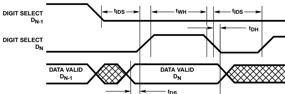
FIGURE 1. MULTIPLEXED INPUT
