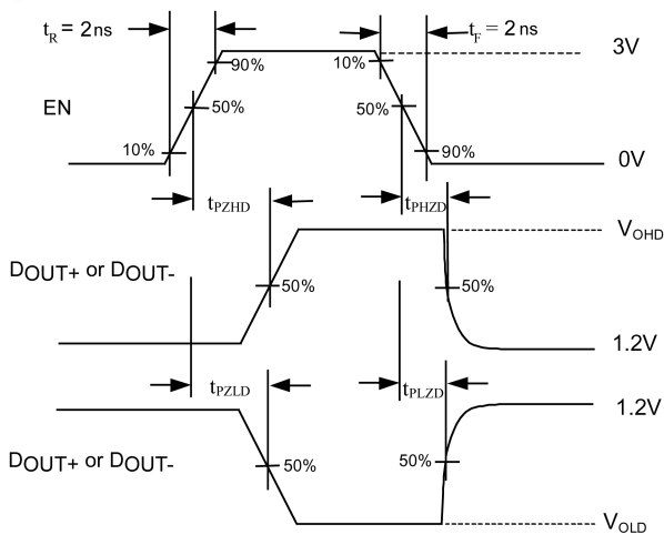
FIGURE 6. Enable and Disable AC Waveforms
