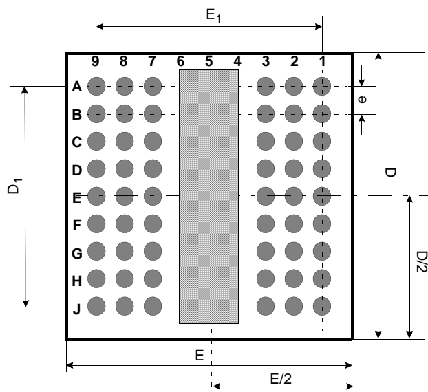
< Bottom View *1 >
