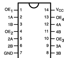
Pin Assignment for SOIC and TSSOP
